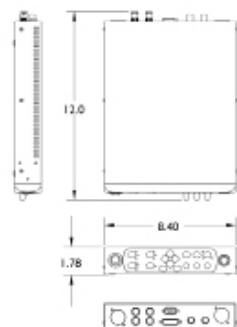
Iconix HD-RH1 Controller
